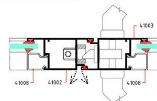
INSIDE Horizontal Section (2)
