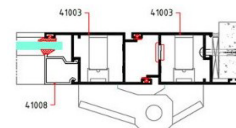
INSIDE Horizontal Section (3)
