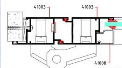
INSIDE Horizontal Section (1)
