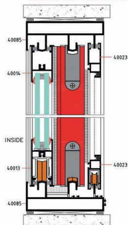
Vertical Section (4-5)
